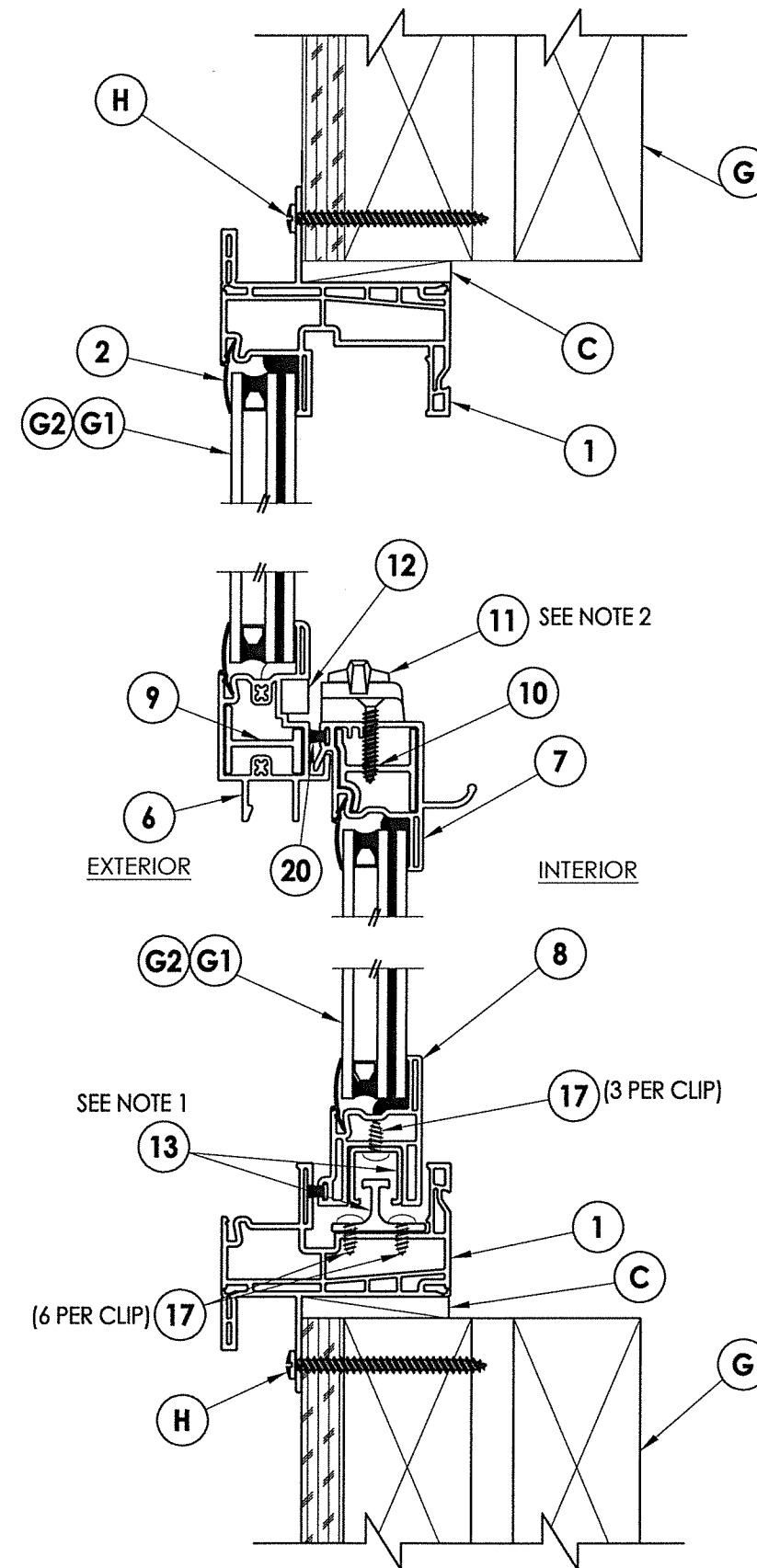
2 VERTICAL CROSS SECTION 3 Stud Construction
